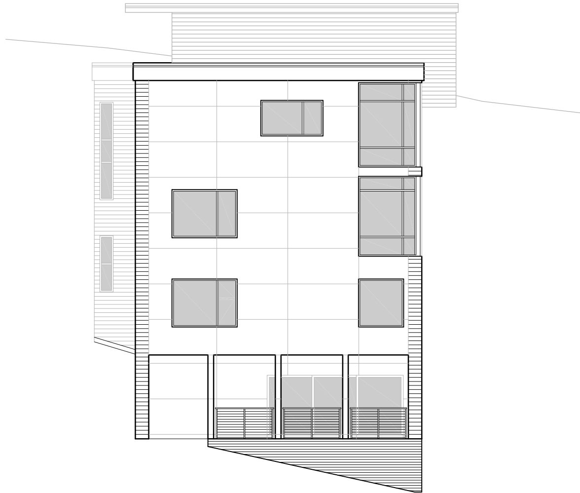
Option #2: East Elevation
